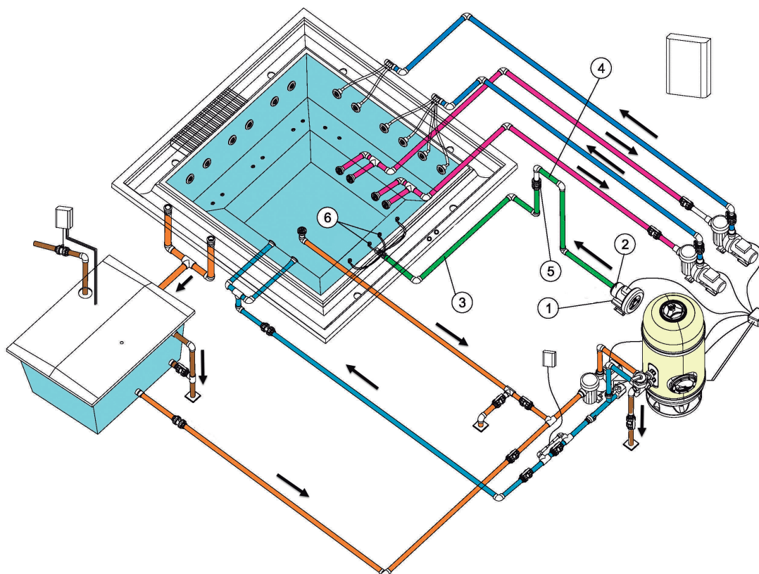
General diagram of Air Spa Massage
