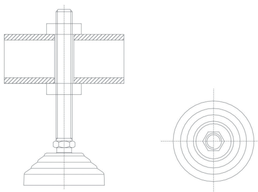
Detail of regulation support.
