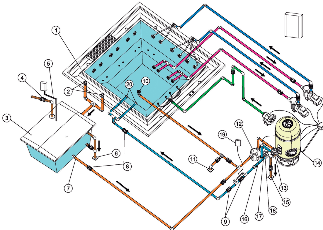
Recirculation diagram of Spa with overflow. Option A
