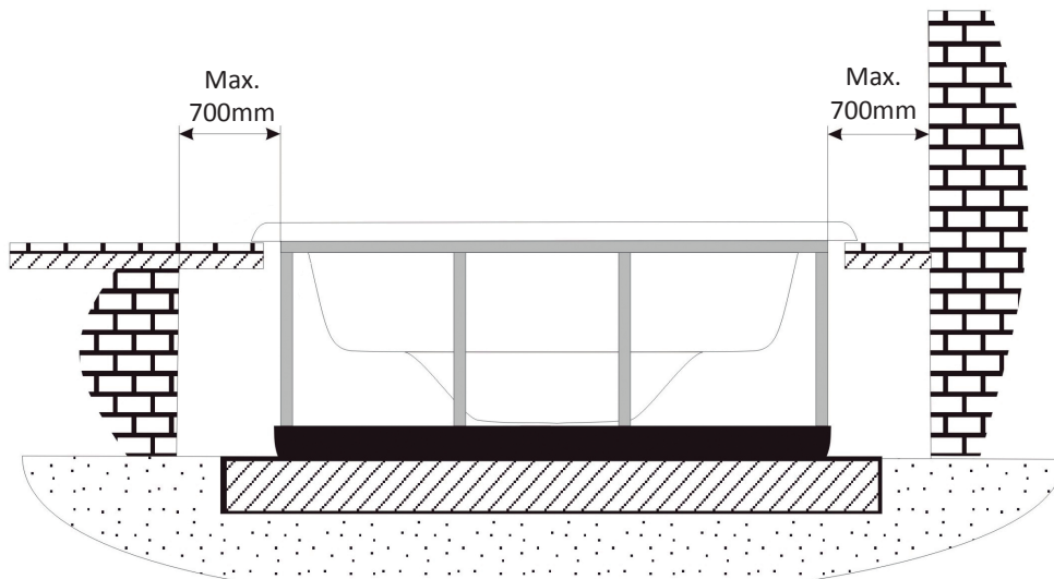
Diagram of minimum distance around the Spa
